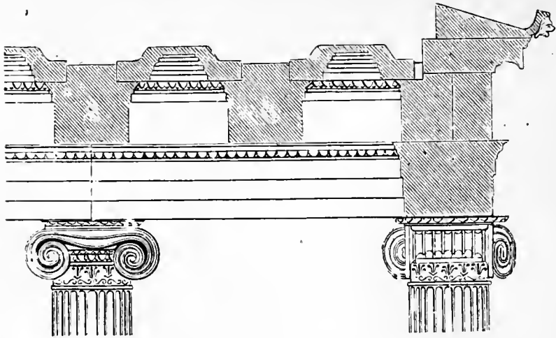
FIG. 88.—SECTION OF THE PORTICO OF THE ERECHTHEUM.
